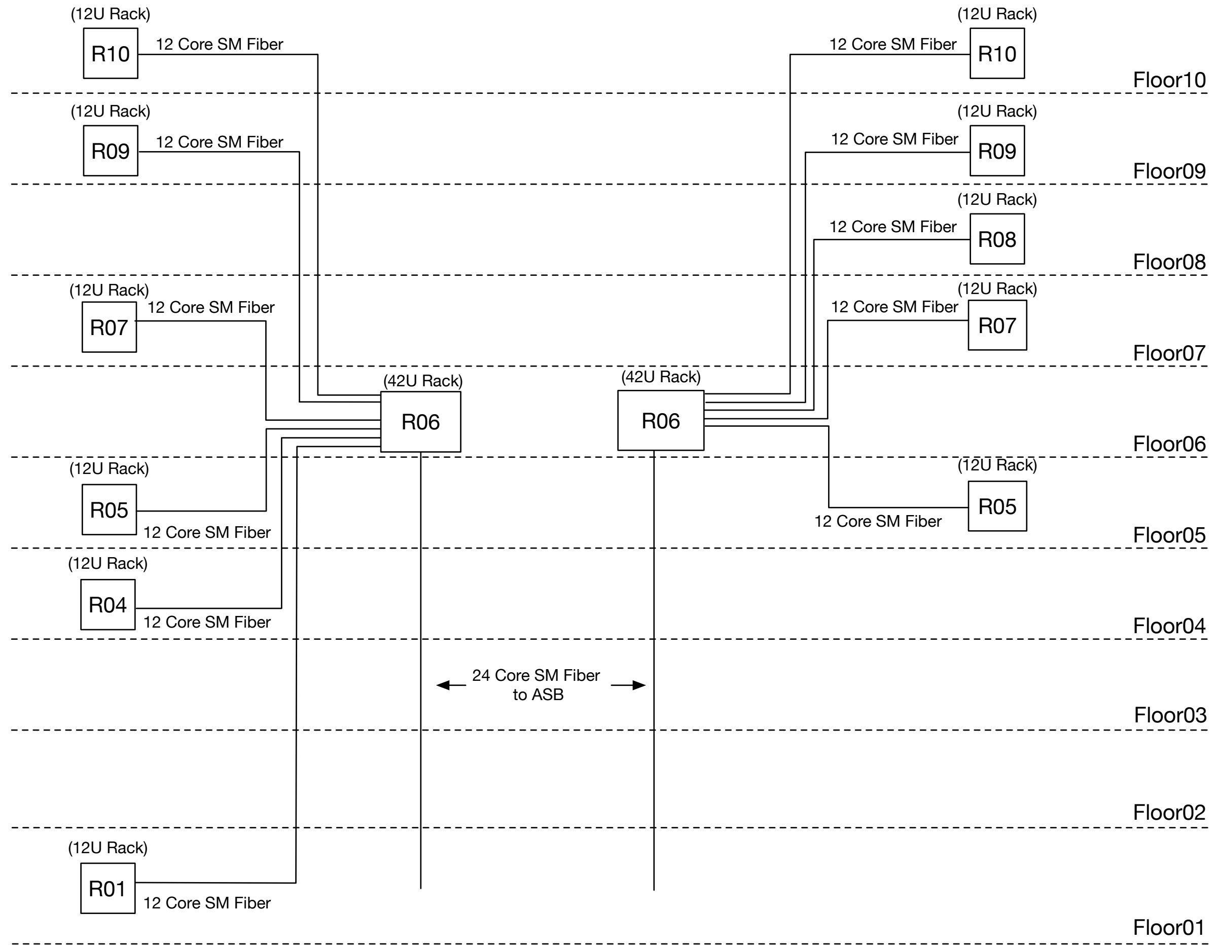
Optical Fiber Diagram
