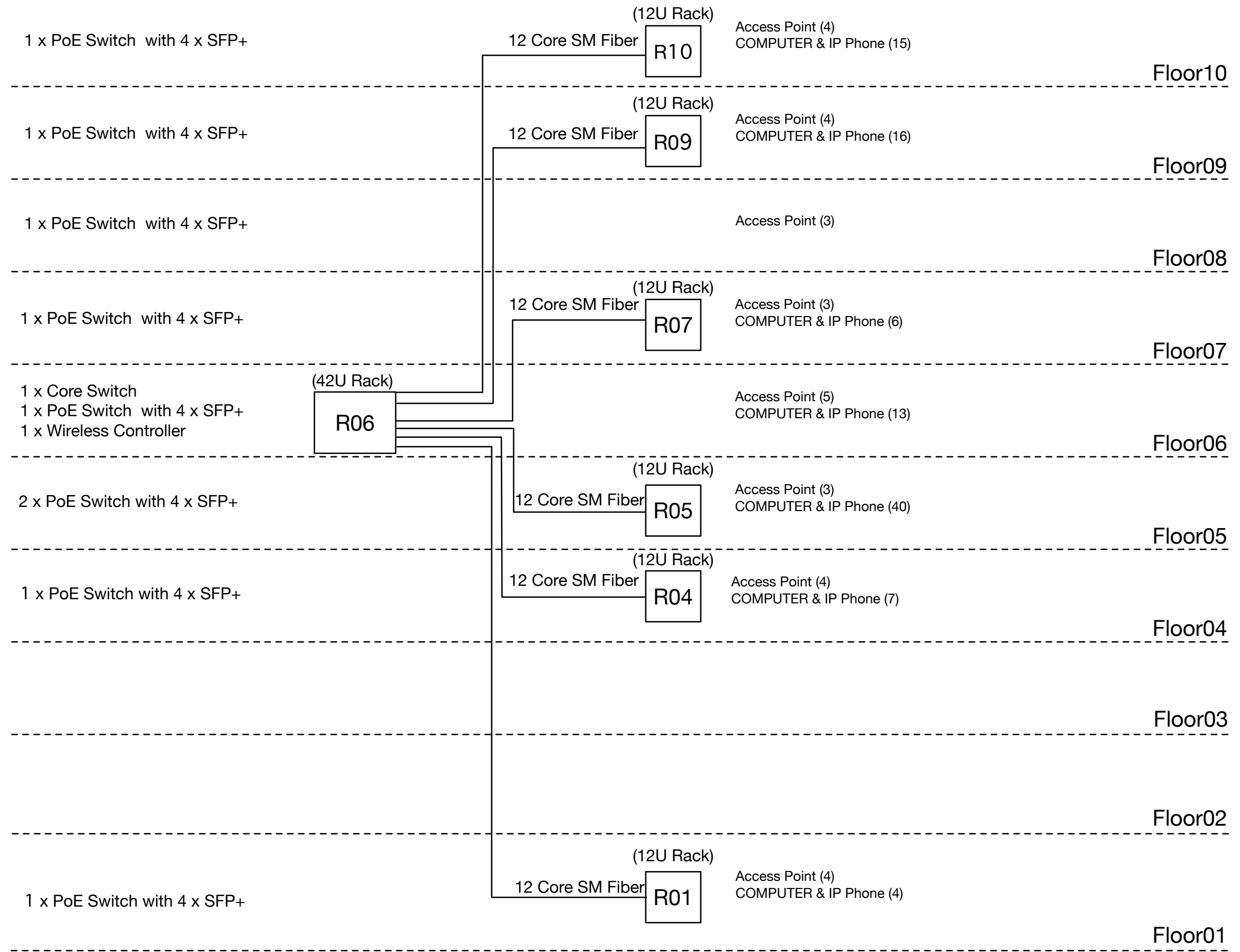
Labs Network Riser Diagram
